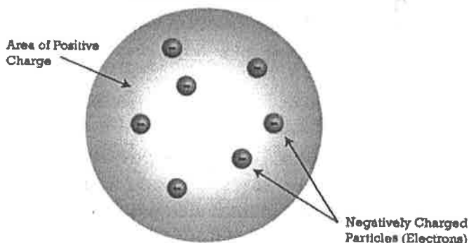
The Plum Pudding Model of an Atom
